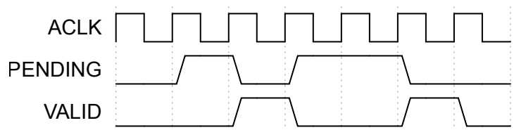
Figure A2.9: Example usage of the PENDING signal
